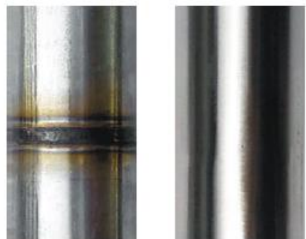
Comparisons of cleaning and polishing of weldings on stainless steel tube: before and after.
